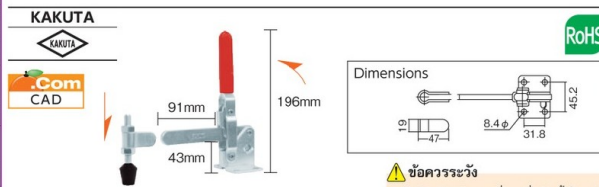
Toggle Clamp (downward press type/vertical handle type) KC-HV550
