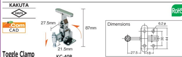
Toggle Clamp (downward press type/vertical handle type)
