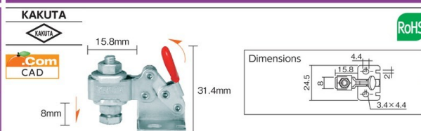
Toggle Clamp (downward press type/vertical handle type) KC-HS-10
