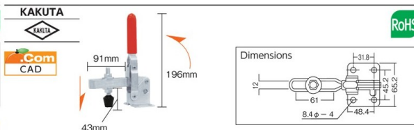
Toggle Clamp (downward press type/vertical handle type) KC-HV650
