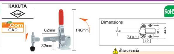
Toggle Clamp (downward press type/vertical handle type) KC-HV350
