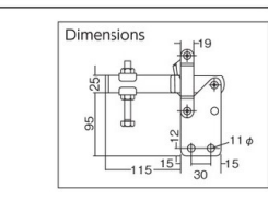
Toggle Clamp (downward press type/vertical handle type)
