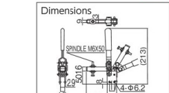
Toggle Clamp (downward press type/vertical handle type)
