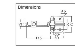
Toggle Clamp (downward press type/vertical handle type)
