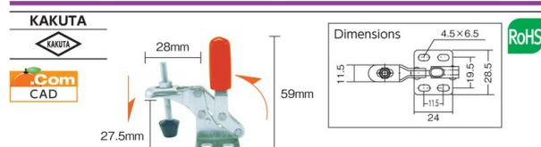
Toggle Clamp (downward press type/vertical handle type)
