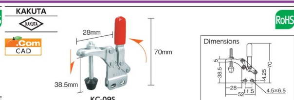
Toggle Clamp (downward press type/vertical handle type)
