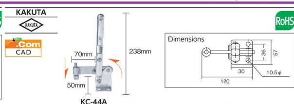
Toggle Clamp (downward press type/vertical handle type)
