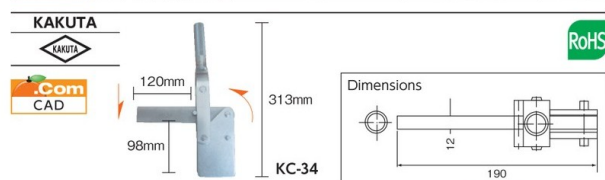
Toggle Clamp (downward press type/vertical handle type)
