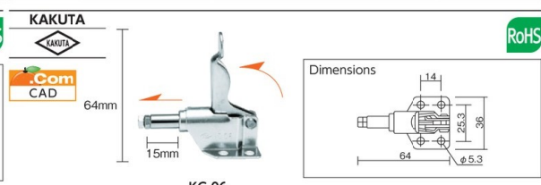
Toggle Clamp (lateral press type)
