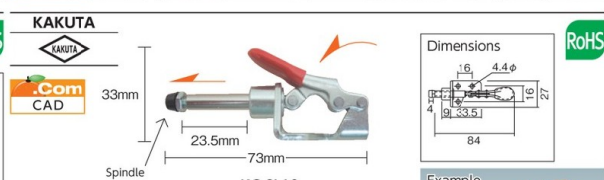
Toggle Clamp (lateral press type)
