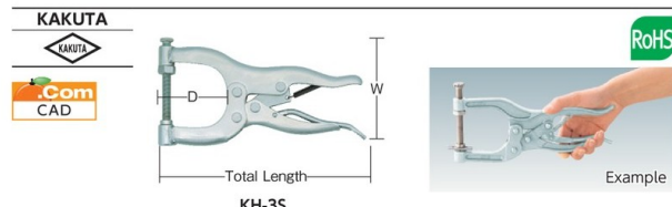
Hand Vice
