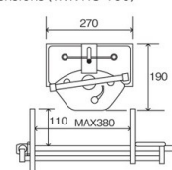
Dimensions (TMVHU-180)
