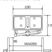
Dimensions (TMVHD-180)
