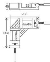
Dimensions (TRAMAV-70)
