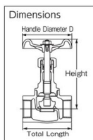
10SJ Type
