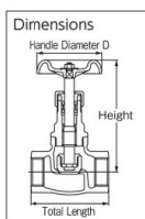
UJ Type
