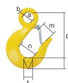
HTL type (Sling Hook HTL)
