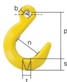
HQ type (Foundry Hook HQ)
