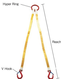
2ILS Type (bifilar suspension)
