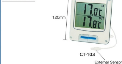
Drip-proof Type Thermometer
