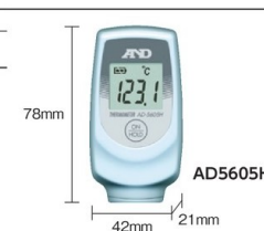
Sensor included (measurement range of the accessory sensor is up to 200°C)
