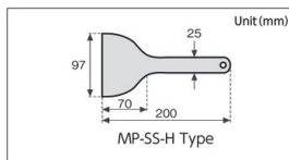
MP Type
