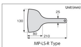
MP-LS-R Type
