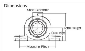
UCP Type
