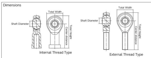
Internal Thread Type External Thread Type
