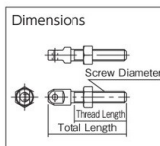
CBS1 (Single Ended Type)
