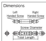
CBD1 (Double Ended Type)
