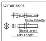
CBS2 (single ended/long type)
