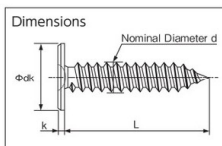
Basic Dimension
