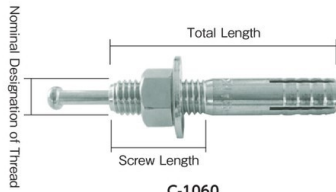
C-1060 (steel)
