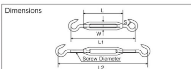
TTB-6H (Hook & Hook type)
