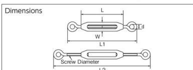
TTB-6E (double eye sided type)
