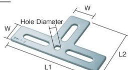
TK24-FT3C (steel) (Chrome Plated Finishing)
