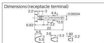
1189ATL (receptacle terminal)
