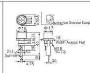
Dimensions (F-130)
