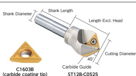
C1603B (carbide coating tip)
