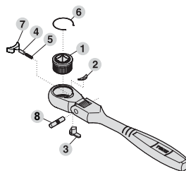
Parts Diagram
