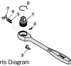
RH3H Parts Diagram
