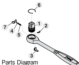
RH3CH Parts Diagram
