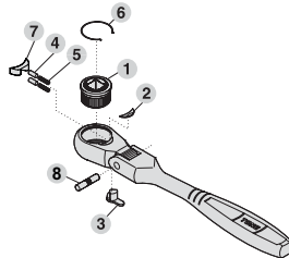
RH3FB Parts Diagram
