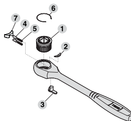
RH3B Parts Diagram
