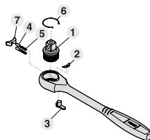
RH4H Parts Diagram
