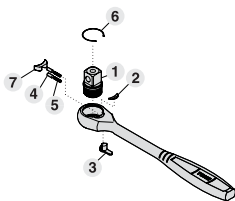
RH4CH Parts Diagram
