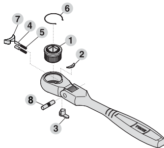
Parts Diagram
