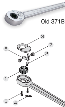
Old 371B Parts Diagram
