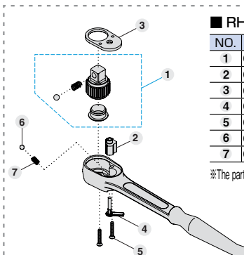
RH40 Parts Diagram
