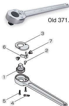
Old 371 Parts Diagram
