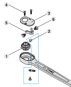
371B Parts Diagram
