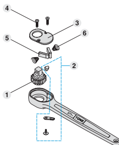
371 Parts Diagram
