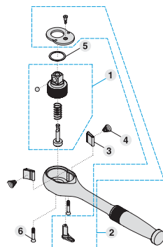
RH43K Parts Diagram
