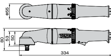
Direction of exhaust can be changed
