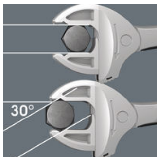
Joker 6004: low return angle
