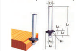
14. Ball bearing beading bit
