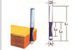
8. Drill point double flush trimming bit
