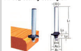
16. Ball bearing cove beading bit
