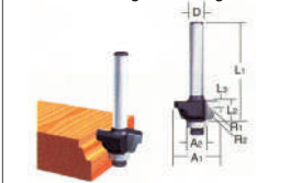
17. Drill point sash router bit For Model 4402
