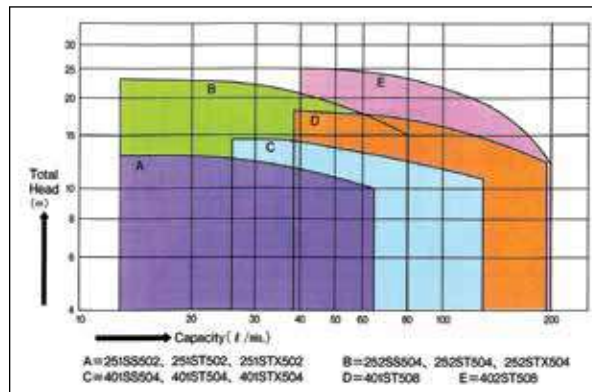
PERFORMANCE CURVE
