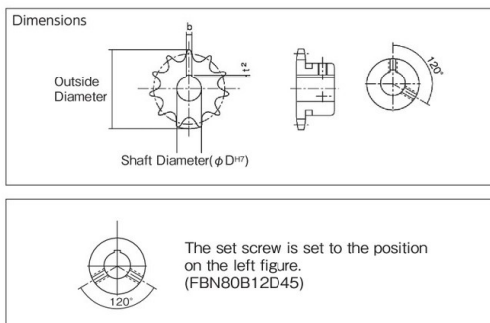
Specs for shaft hole processing
